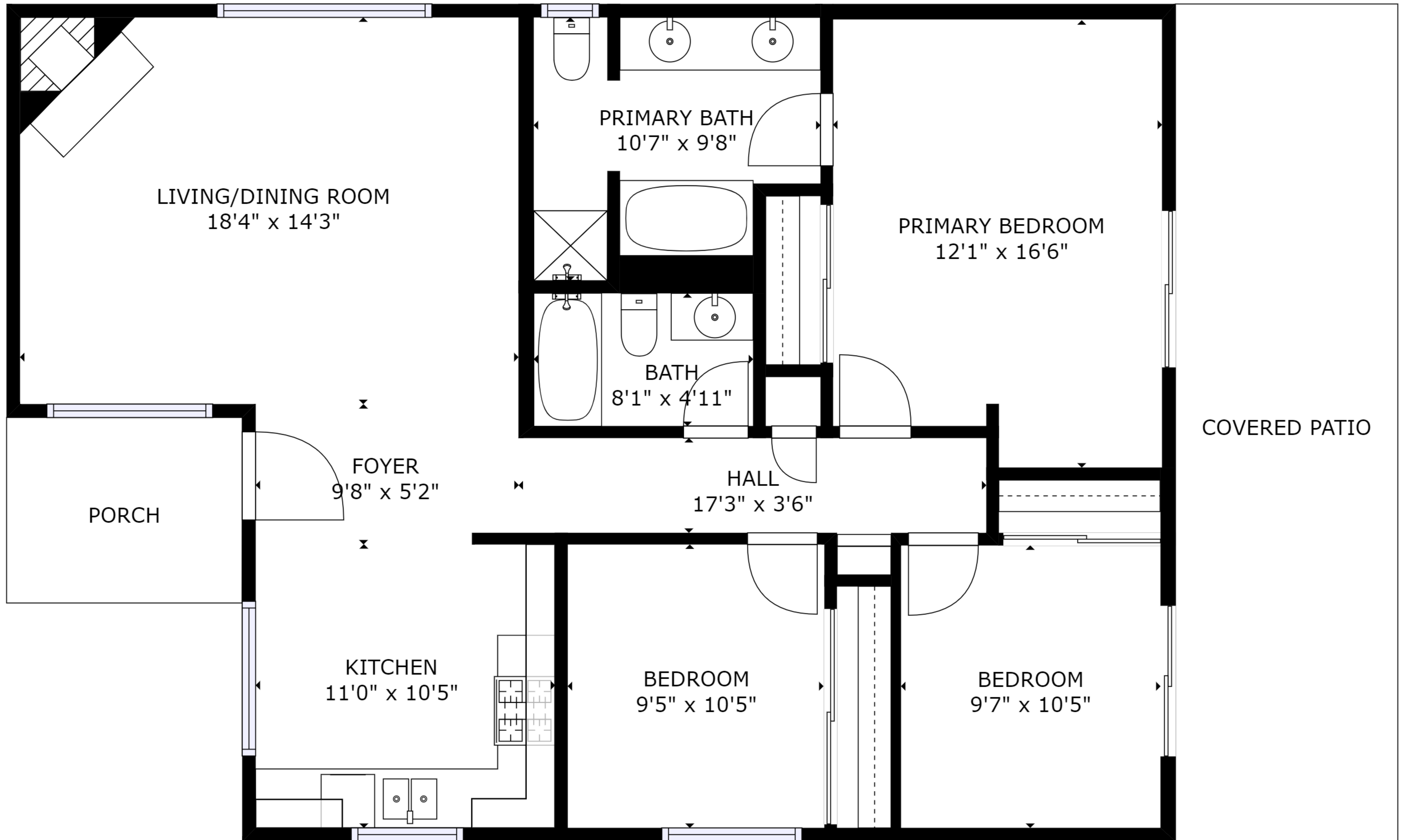
FLOOR 1
