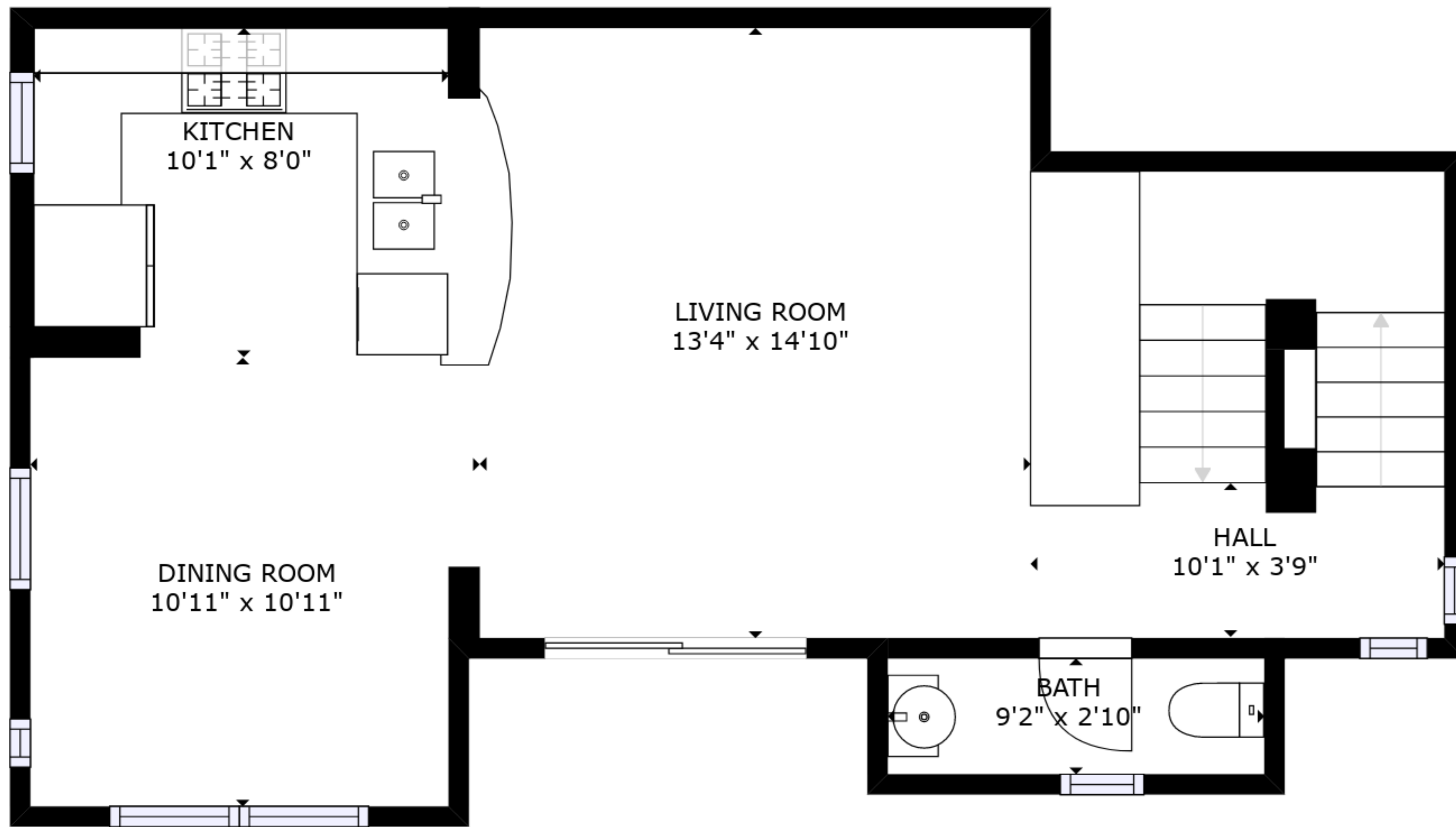
FLOOR 2
