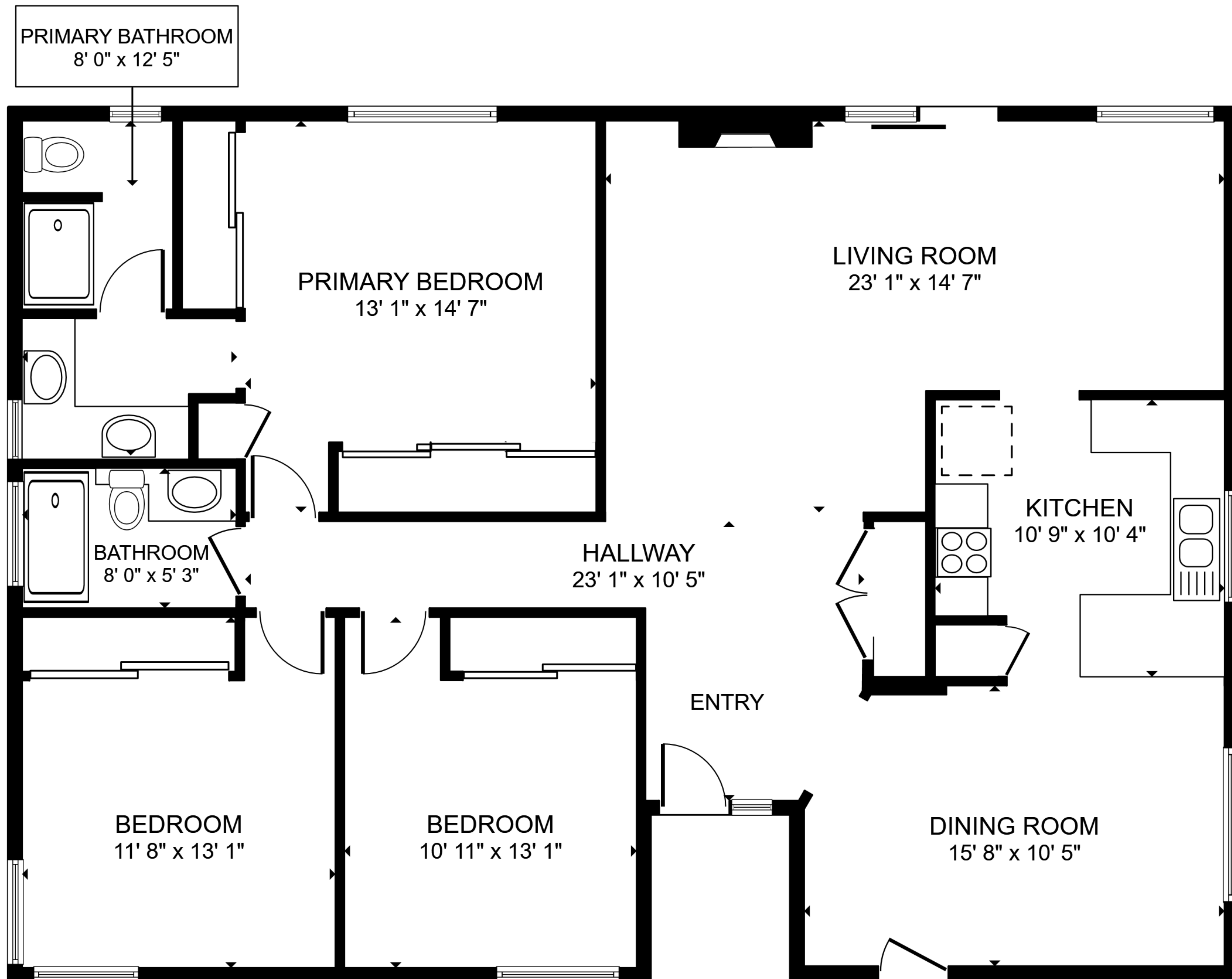
FLOOR PLAN
