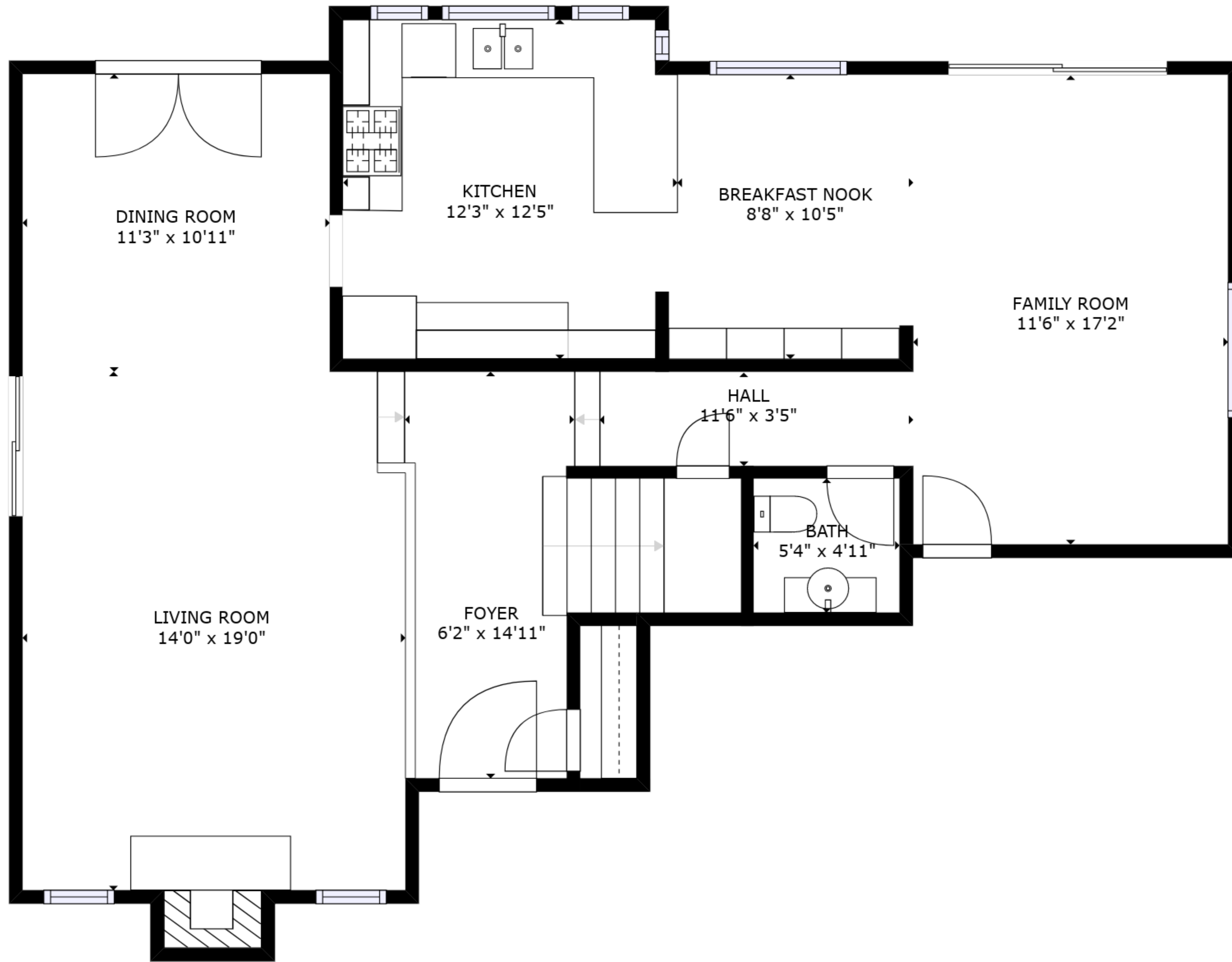
FLOOR 1
