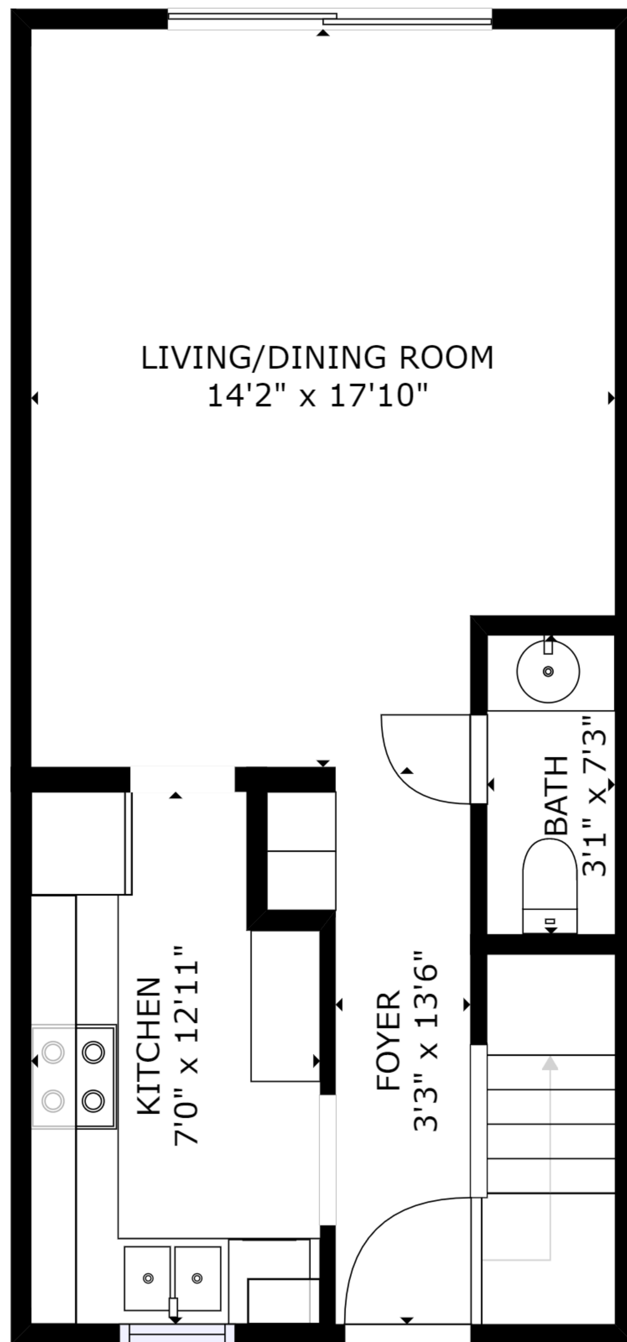
FLOOR 1
