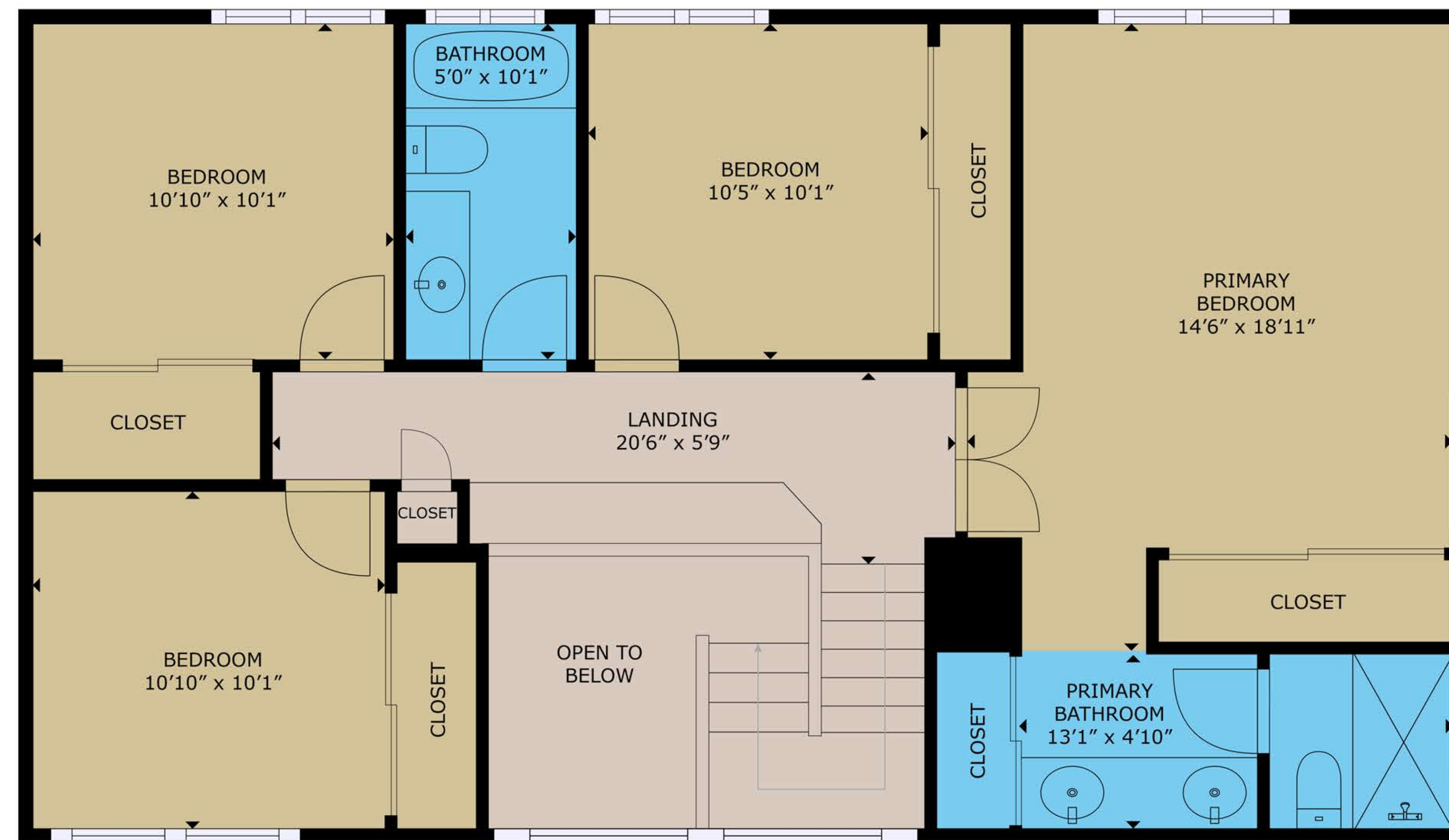
FLOOR 2
