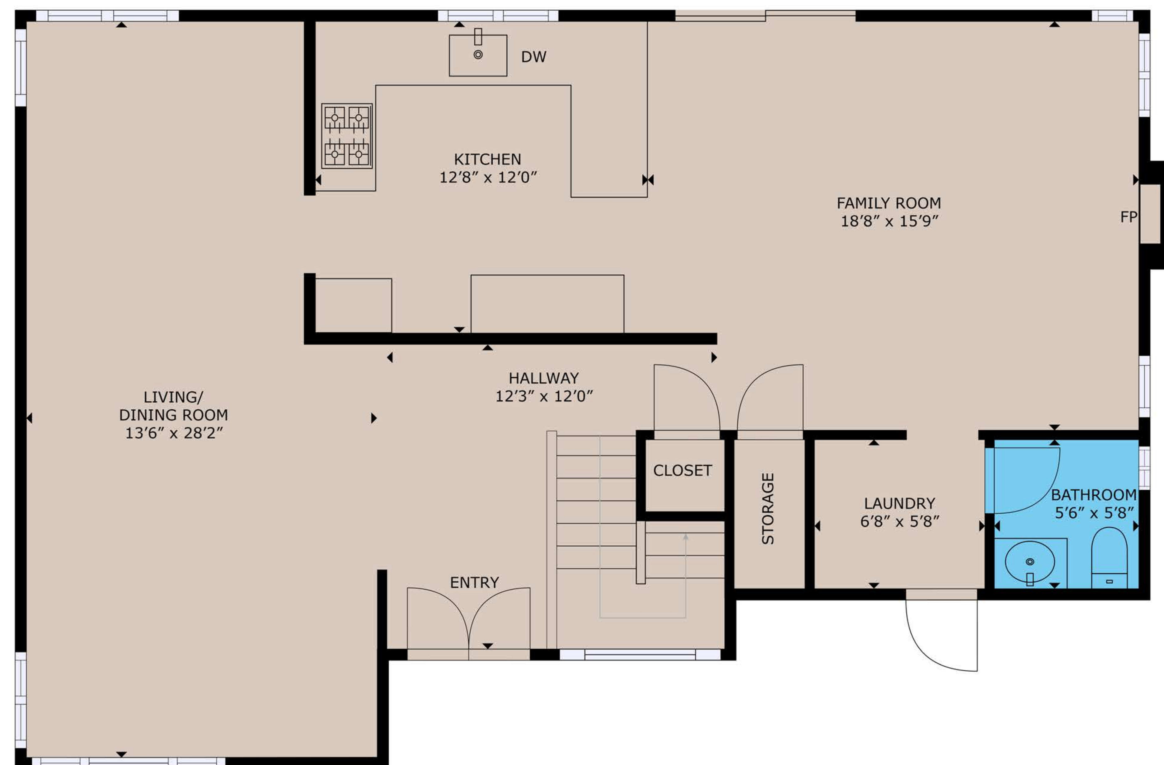
FLOOR 1
