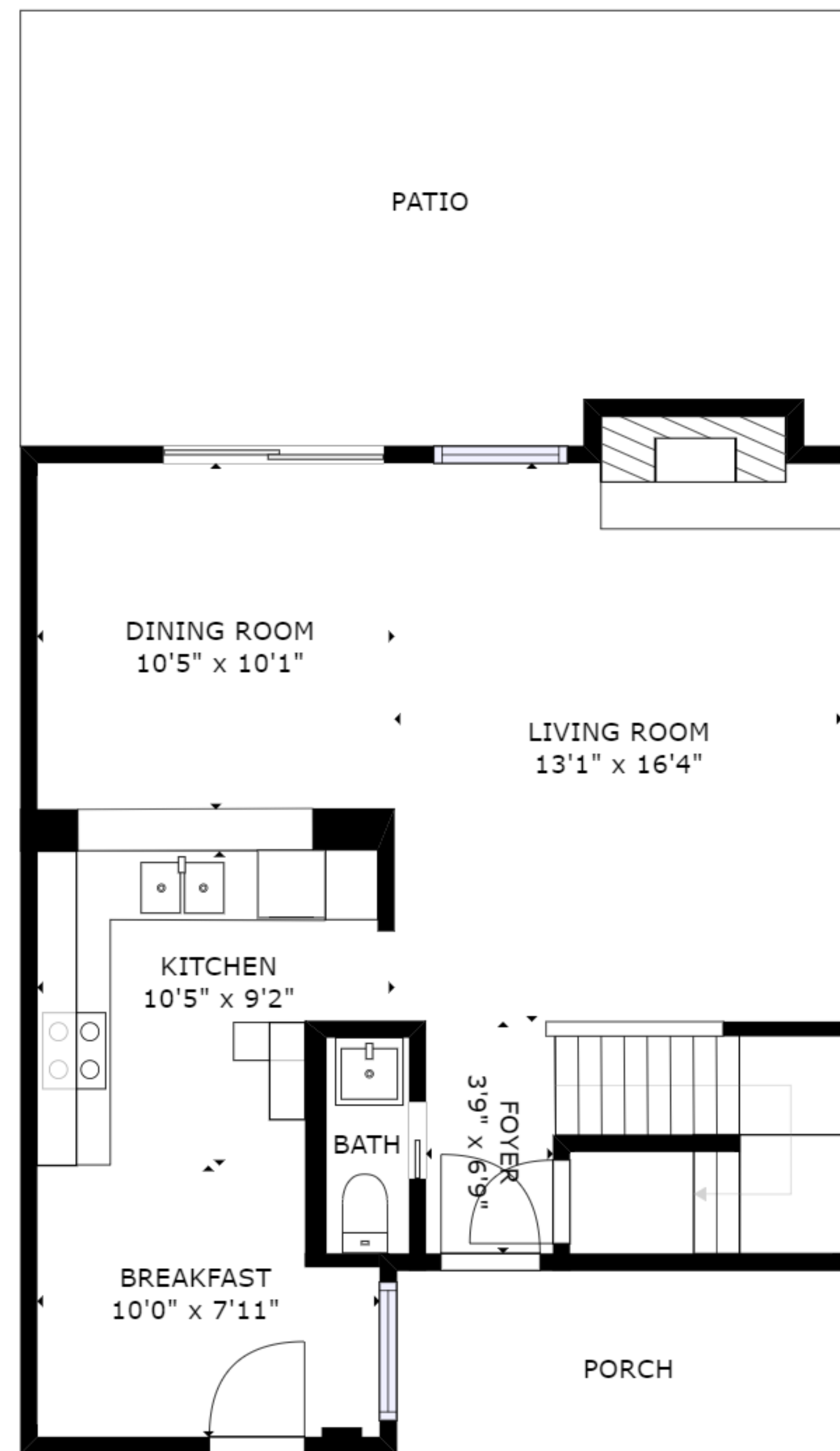
FLOOR 1
