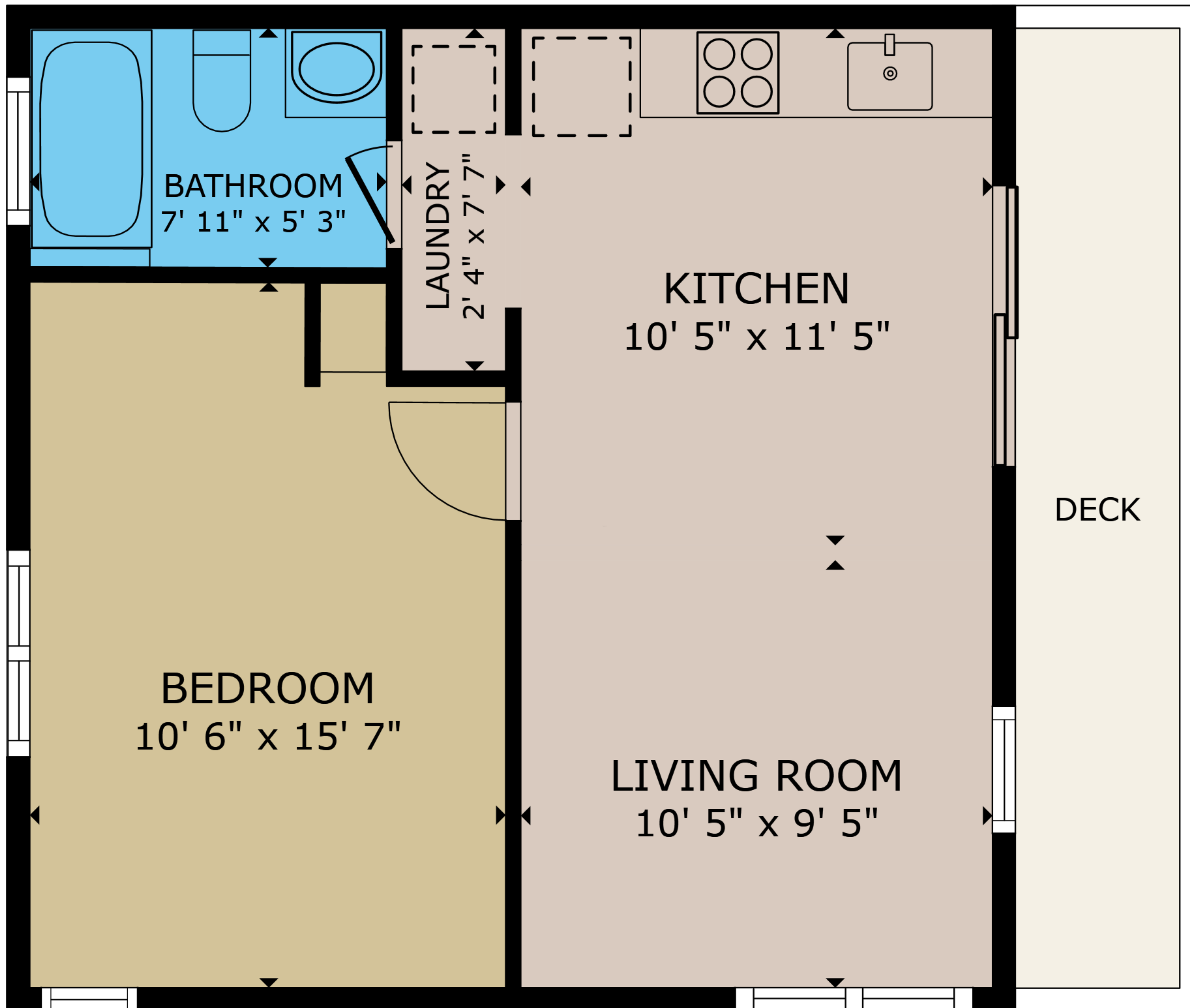
FLOOR PLAN
