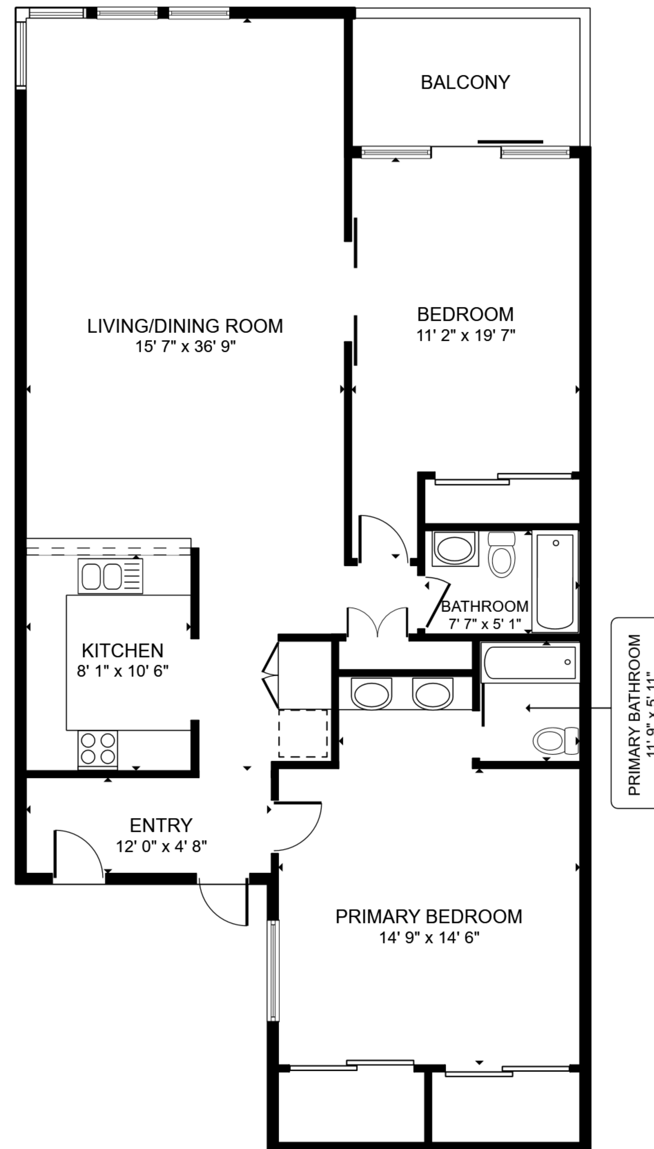
FLOOR PLAN
