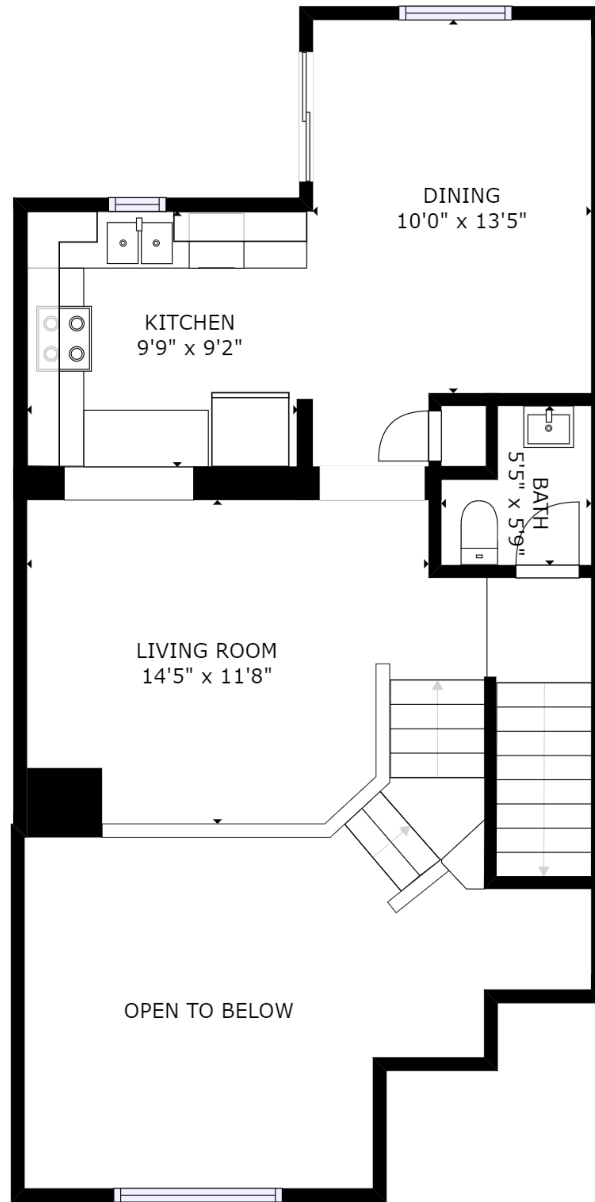
FLOOR 1
