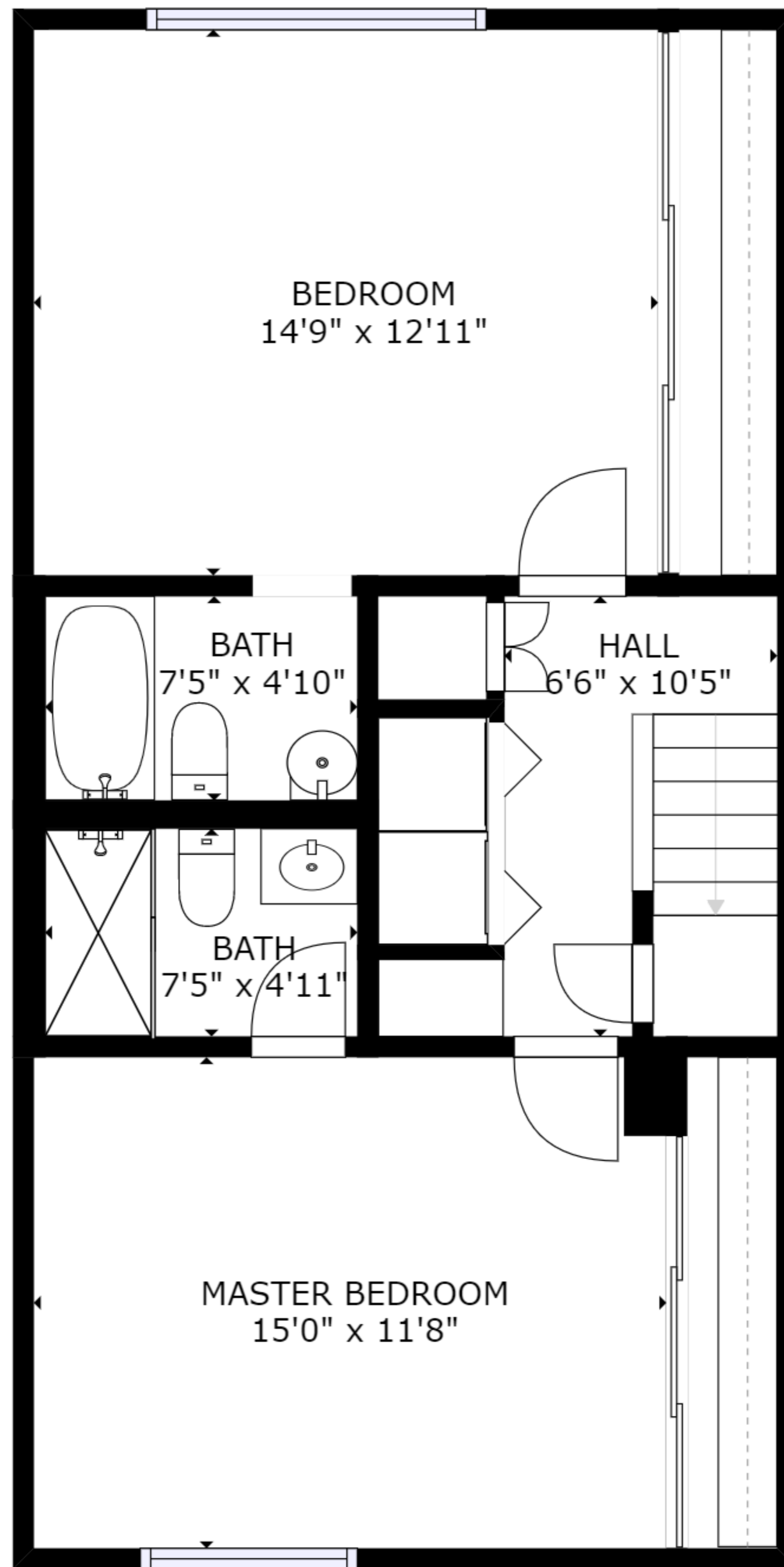
FLOOR 1
